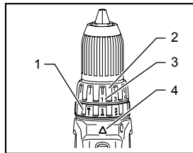
1. Action mode changing ring 2. Adjusting ring 3. Graduation 4. Arrow
